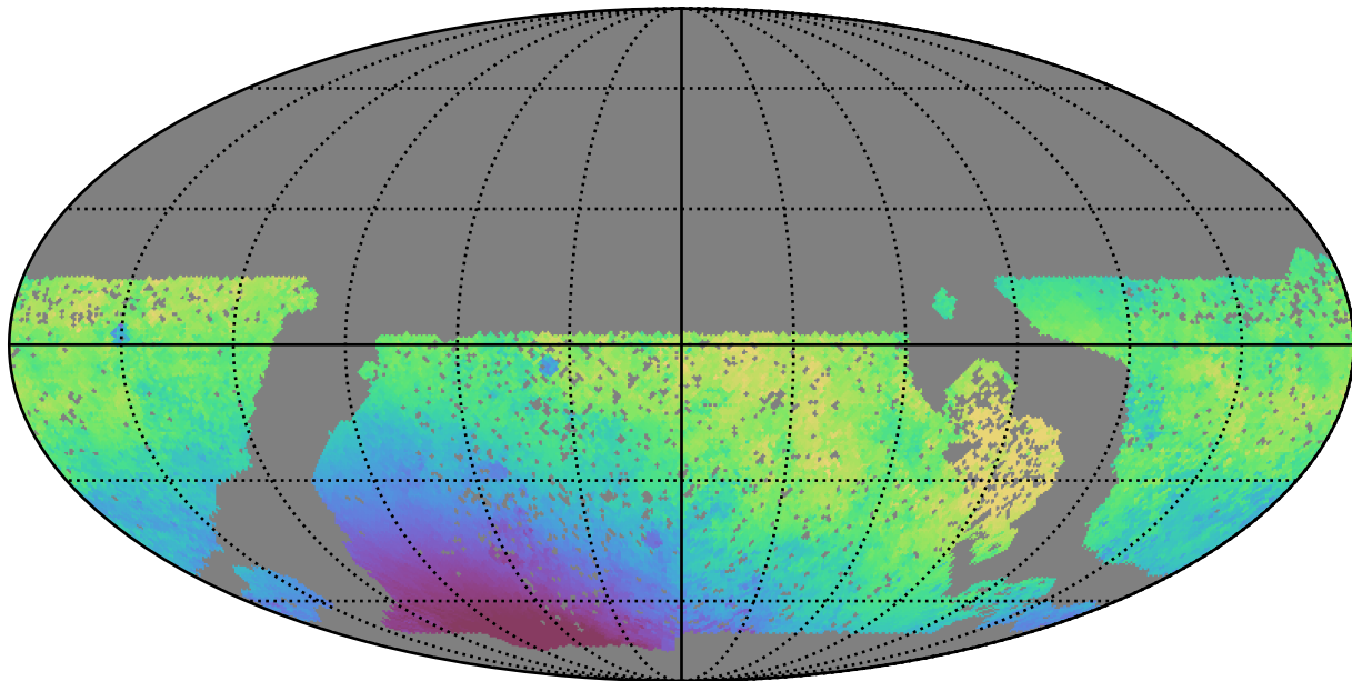
baseline_v3.0_10yrs WFD u band: Median moonDistance
