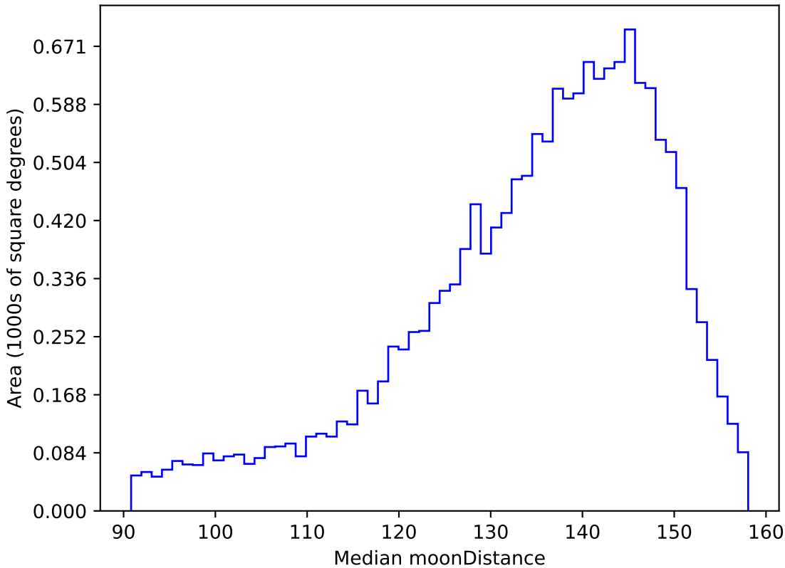
baseline_v3.0_10yrs WFD u band: Median moonDistance
