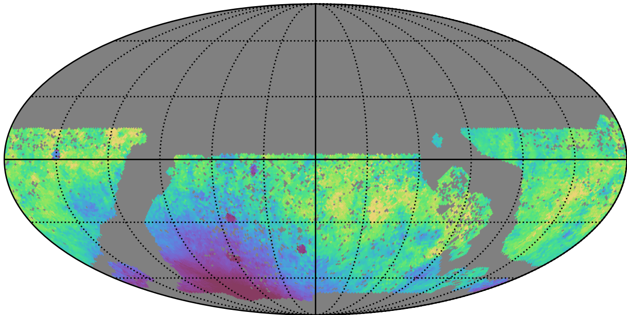
baseline_v3.0_10yrs WFD r band: Median moonDistance
