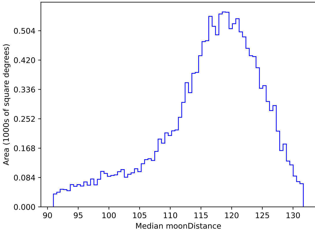
baseline_v3.0_10yrs WFD r band: Median moonDistance
