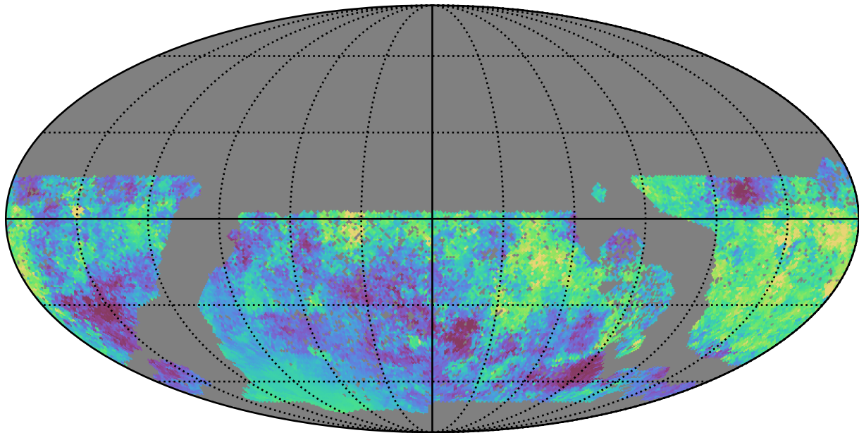
baseline_v3.0_10yrs WFD i band: Median moonDistance
