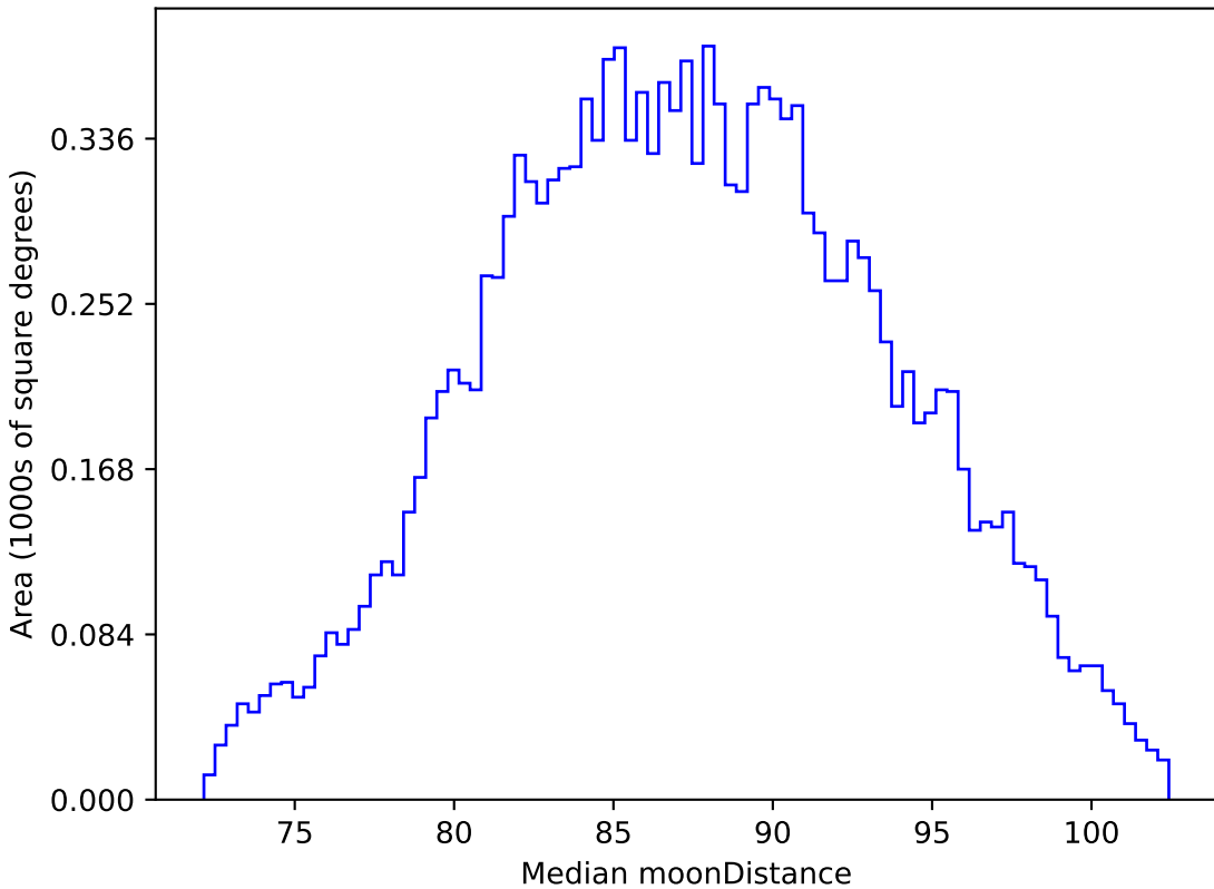
baseline_v3.0_10yrs WFD i band: Median moonDistance
