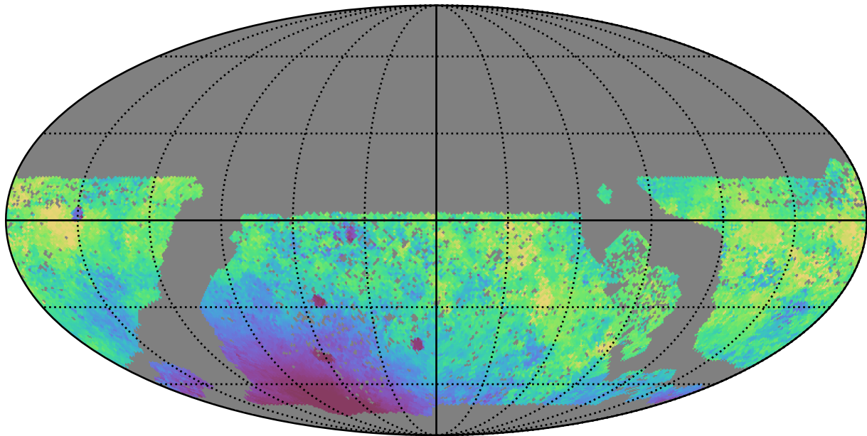
baseline_v3.0_10yrs WFD g band: Median moonDistance
