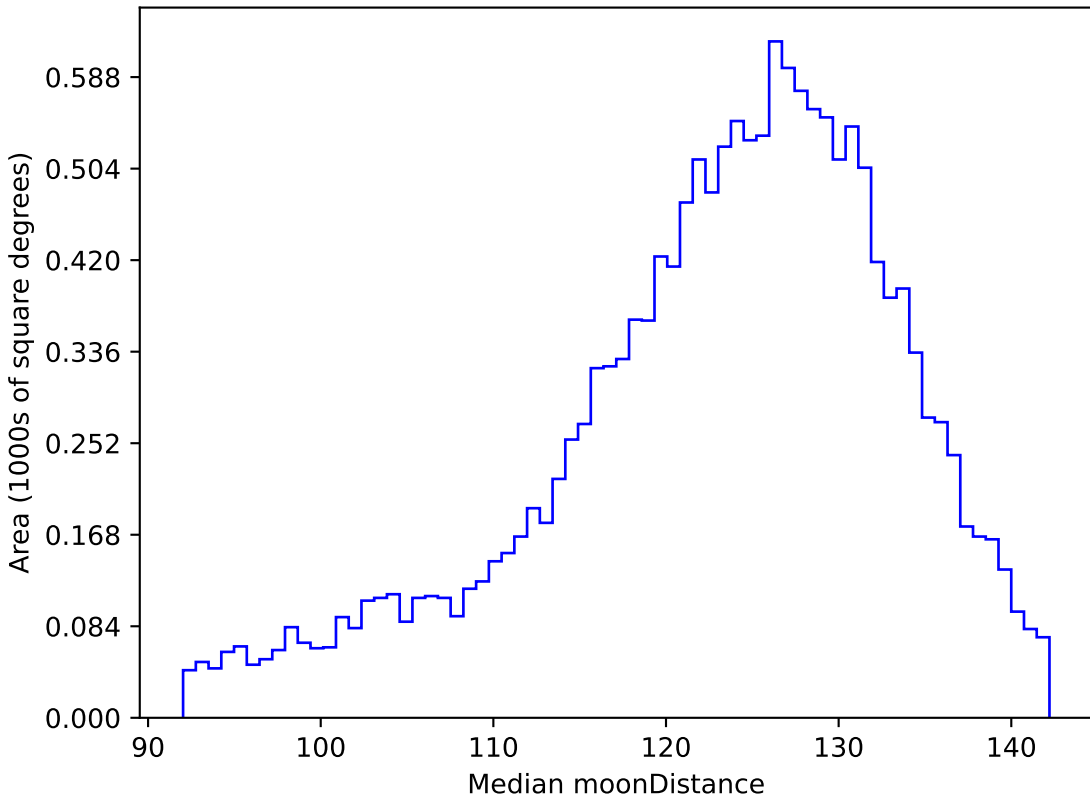
baseline_v3.0_10yrs WFD g band: Median moonDistance
