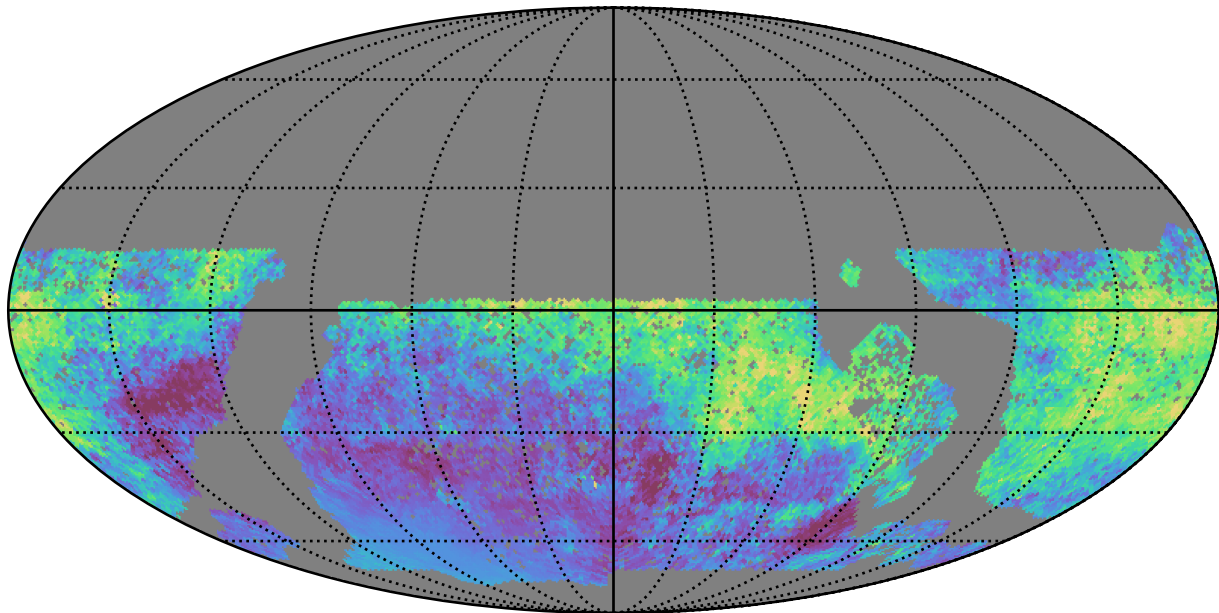
baseline_v3.0_10yrs WFD all bands: Median moonDistance
