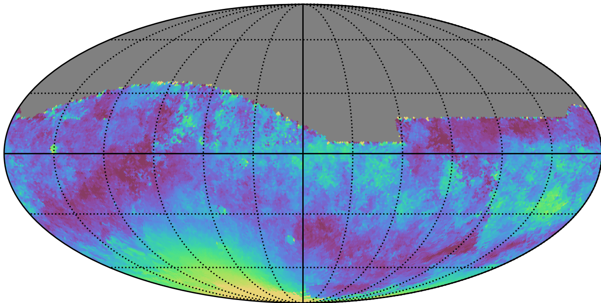
baseline_v3.0_10yrs All sky z band: Median moonDistance
