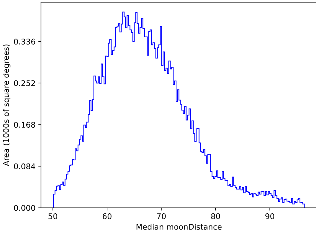
baseline_v3.0_10yrs All sky z band: Median moonDistance
