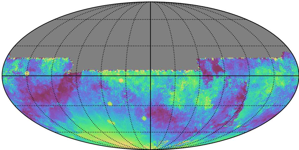
baseline_v3.0_10yrs All sky y band: Median moonDistance
