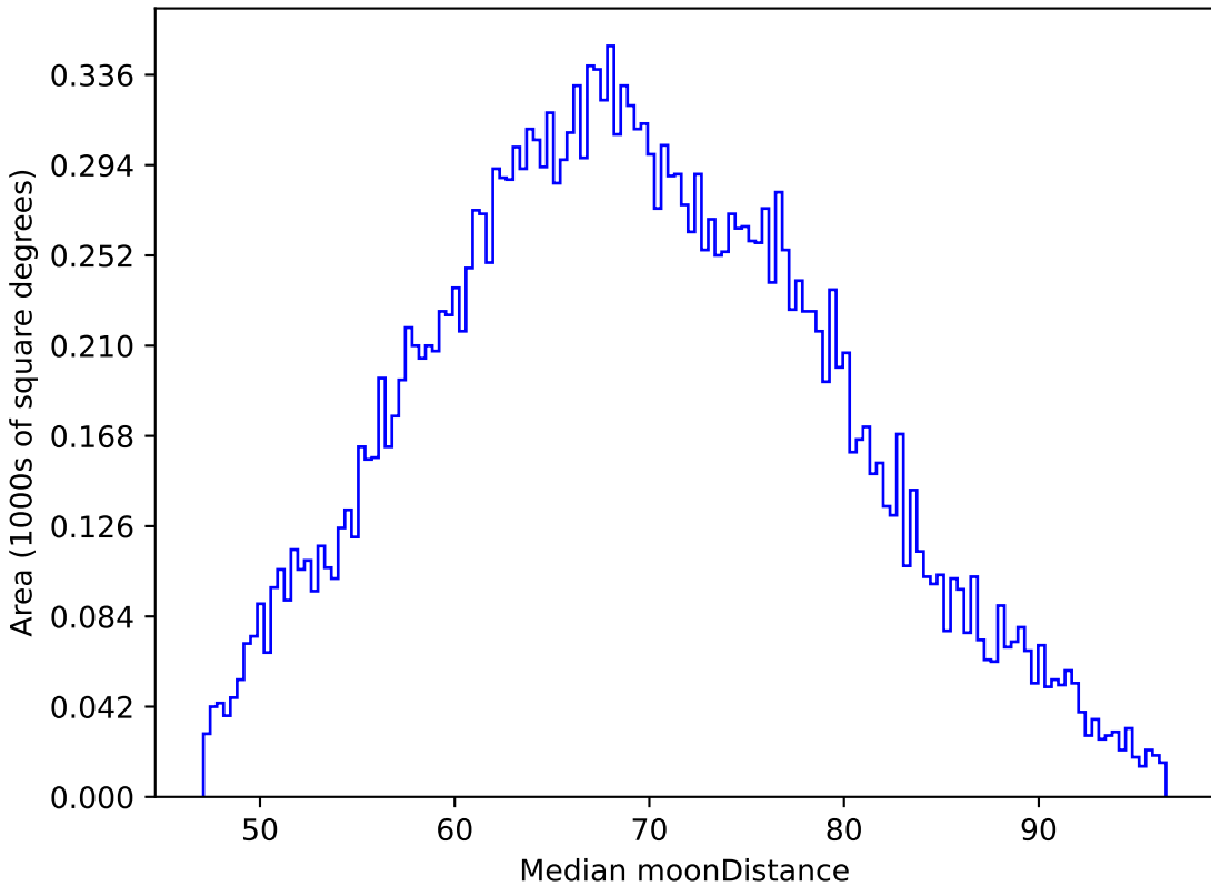
baseline_v3.0_10yrs All sky y band: Median moonDistance
