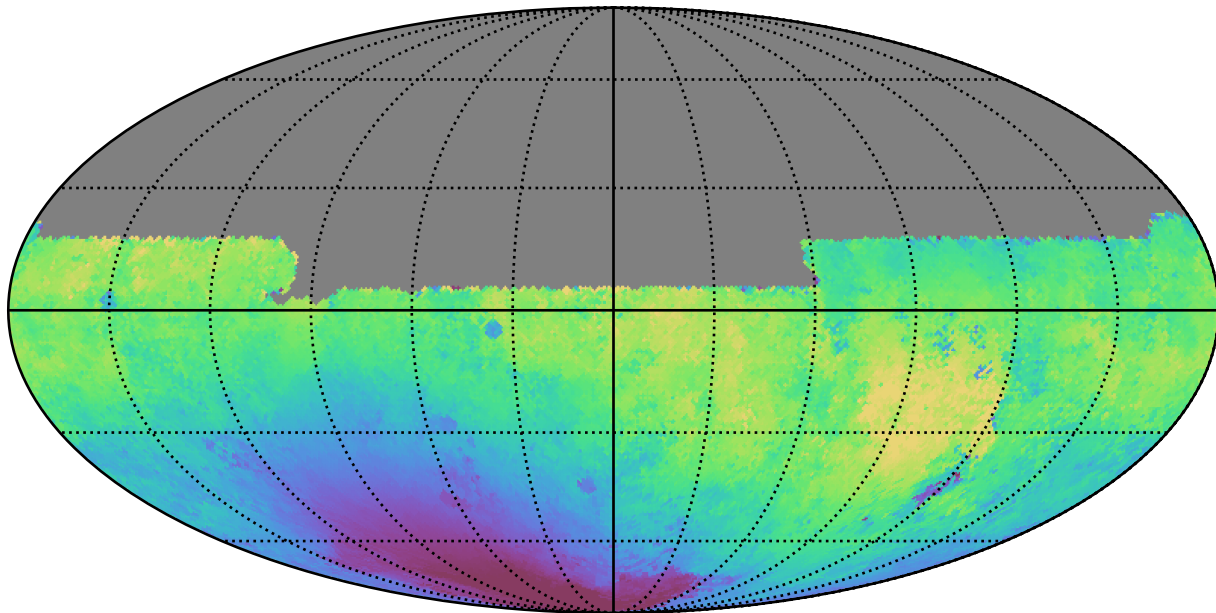
baseline_v3.0_10yrs All sky u band: Median moonDistance
