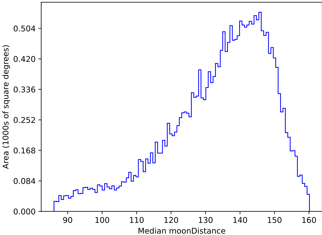
baseline_v3.0_10yrs All sky u band: Median moonDistance
