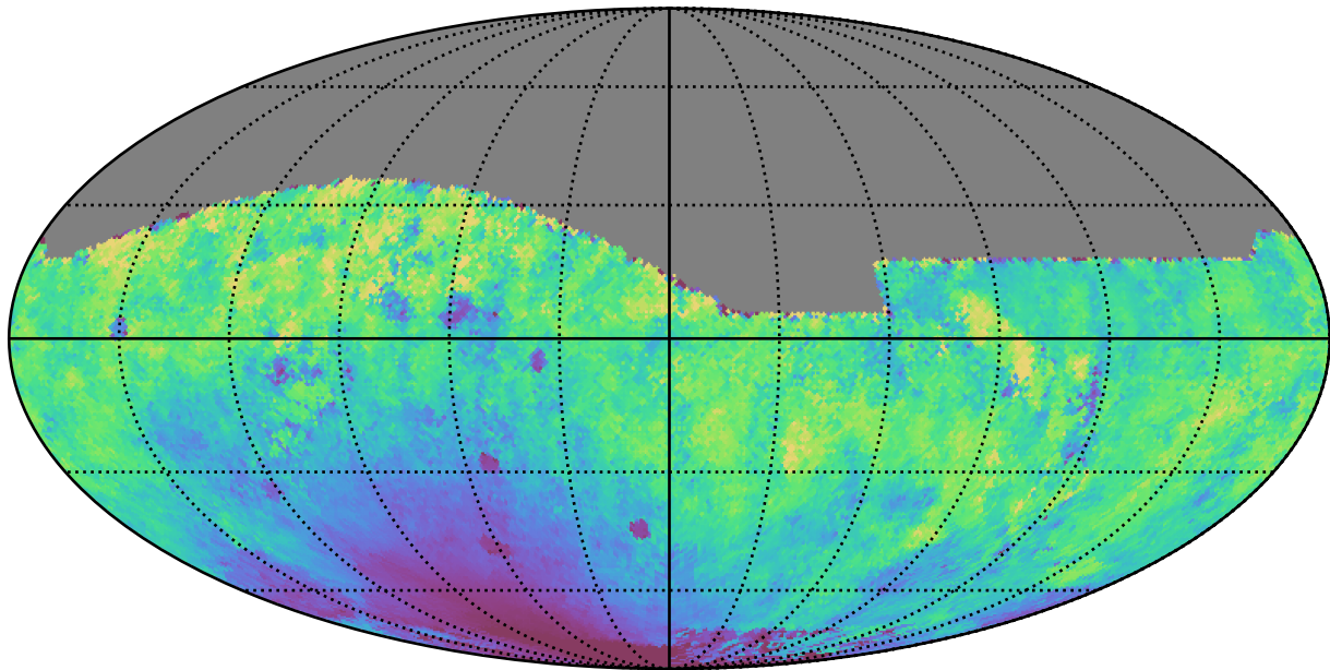
baseline_v3.0_10yrs All sky r band: Median moonDistance
