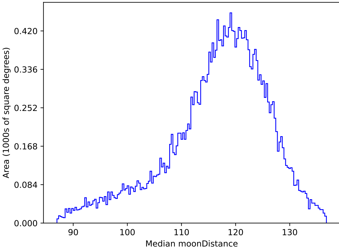
baseline_v3.0_10yrs All sky r band: Median moonDistance
