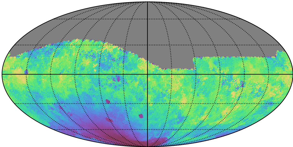
baseline_v3.0_10yrs All sky g band: Median moonDistance
