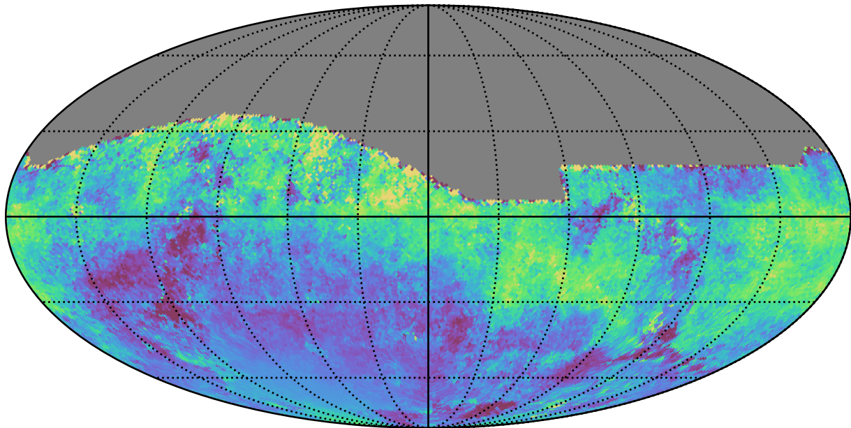
baseline_v3.0_10yrs All sky all bands: Median moonDistance
