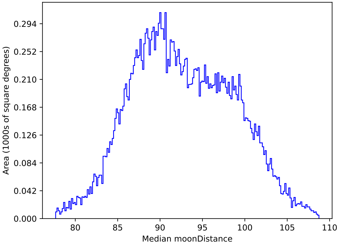
baseline_v3.0_10yrs All sky all bands: Median moonDistance
