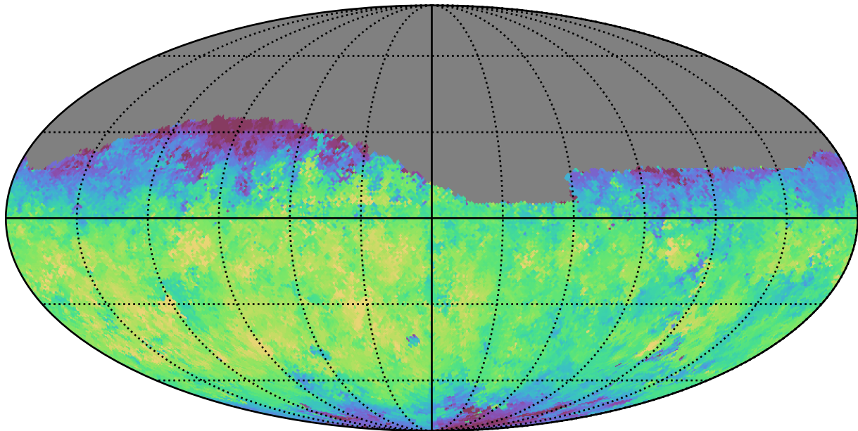
baseline_v3.0_10yrs Yr 1 z band: Median fiveSigmaDepth
