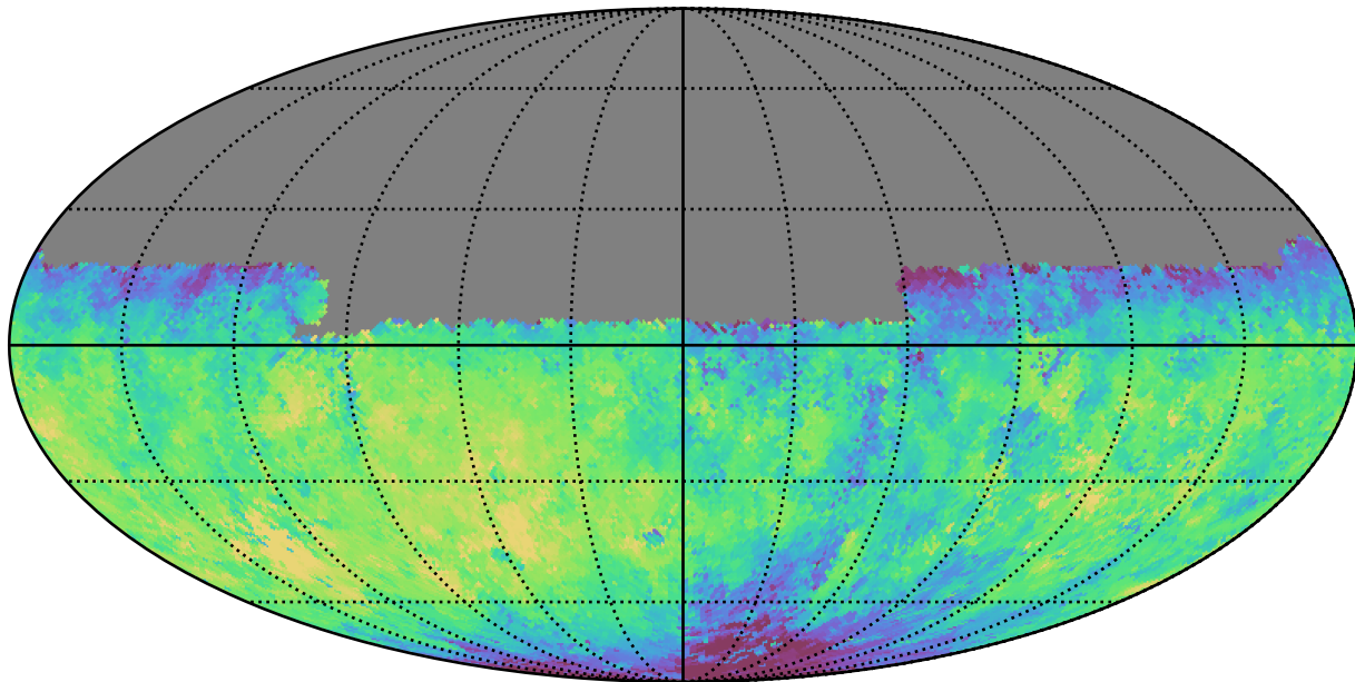
baseline_v3.0_10yrs Yr 1 y band: Median fiveSigmaDepth
