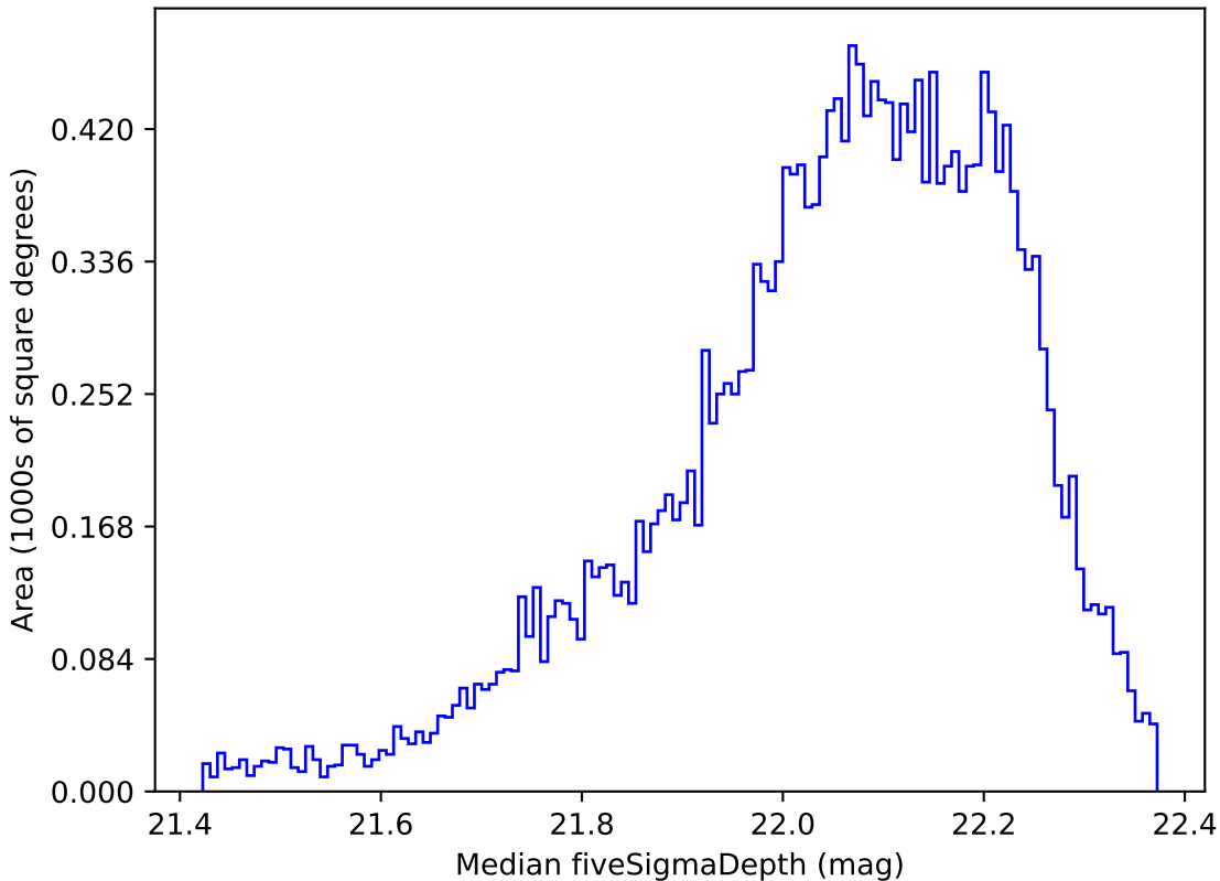
baseline_v3.0_10yrs Yr 1 y band: Median fiveSigmaDepth
