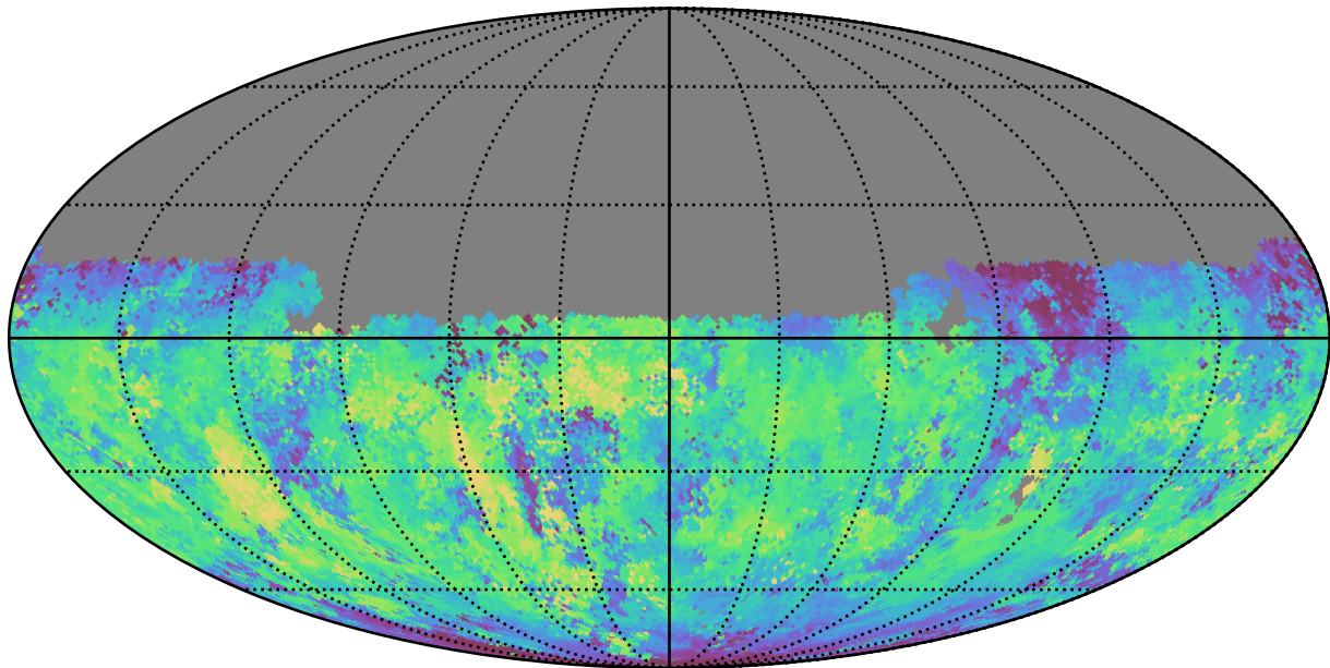
baseline_v3.0_10yrs Yr 1 u band: Median fiveSigmaDepth
