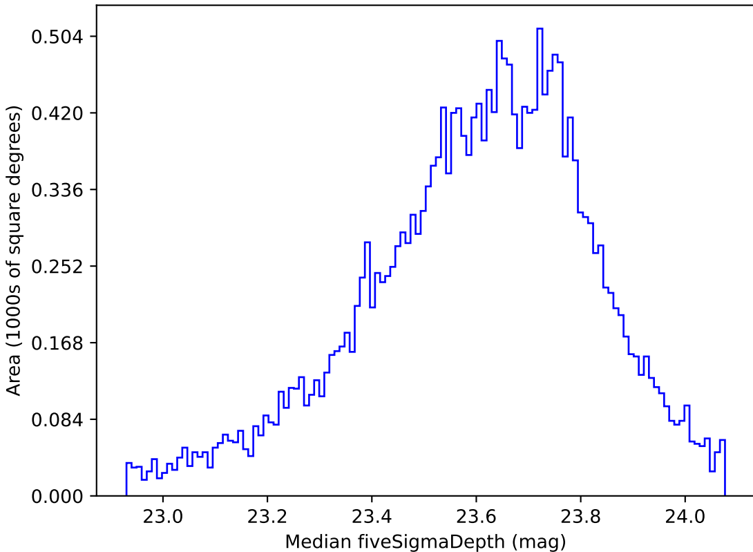
baseline_v3.0_10yrs Yr 1 u band: Median fiveSigmaDepth
