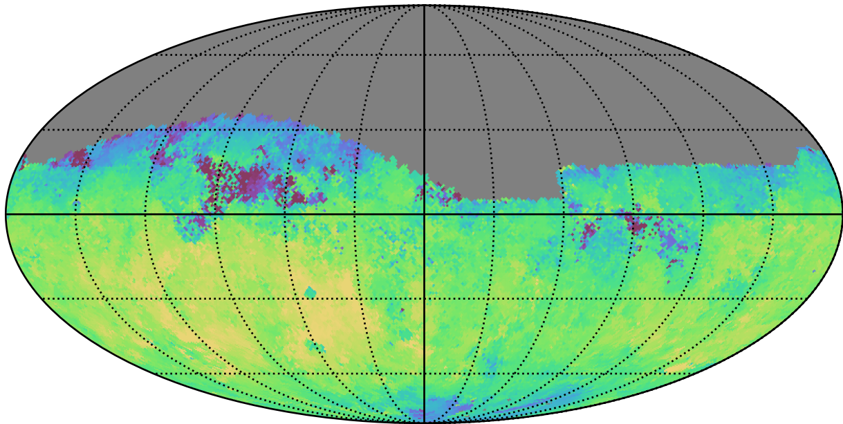
baseline_v3.0_10yrs Yr 1 r band: Median fiveSigmaDepth
