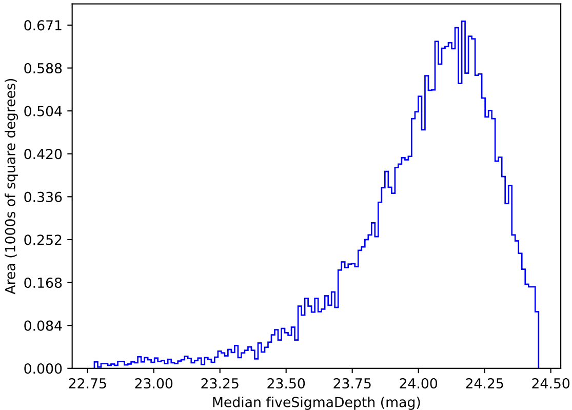
baseline_v3.0_10yrs Yr 1 r band: Median fiveSigmaDepth
