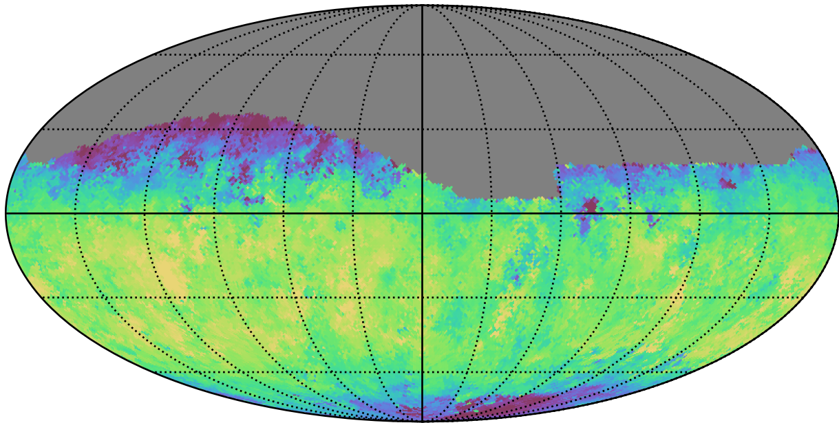
baseline_v3.0_10yrs Yr 1 i band: Median fiveSigmaDepth
