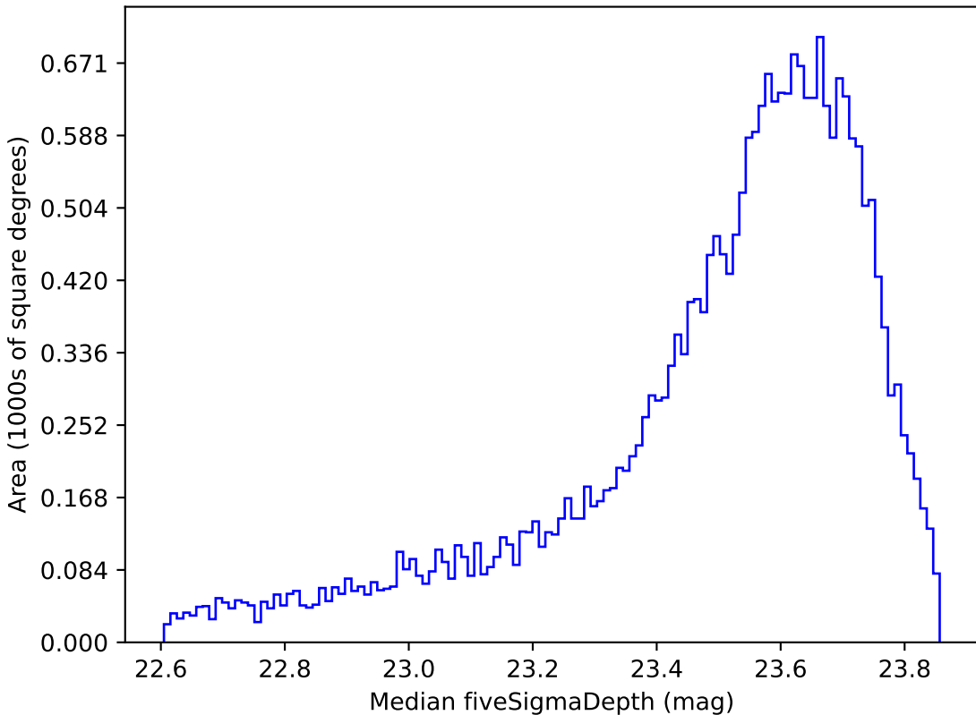
baseline_v3.0_10yrs Yr 1 i band: Median fiveSigmaDepth
