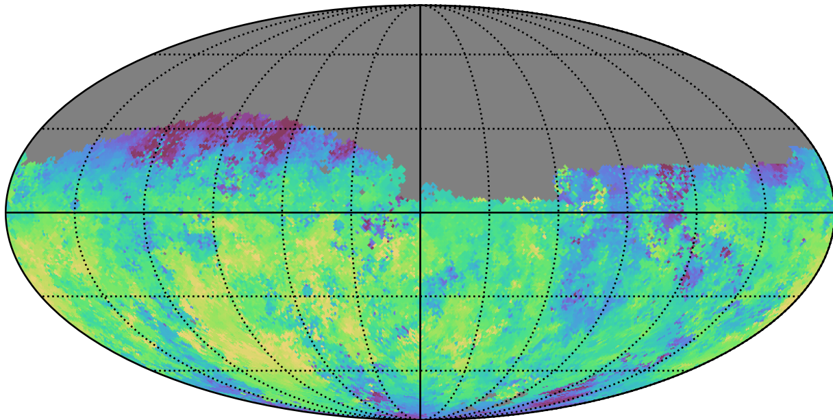
baseline_v3.0_10yrs Yr 1 g band: Median fiveSigmaDepth
