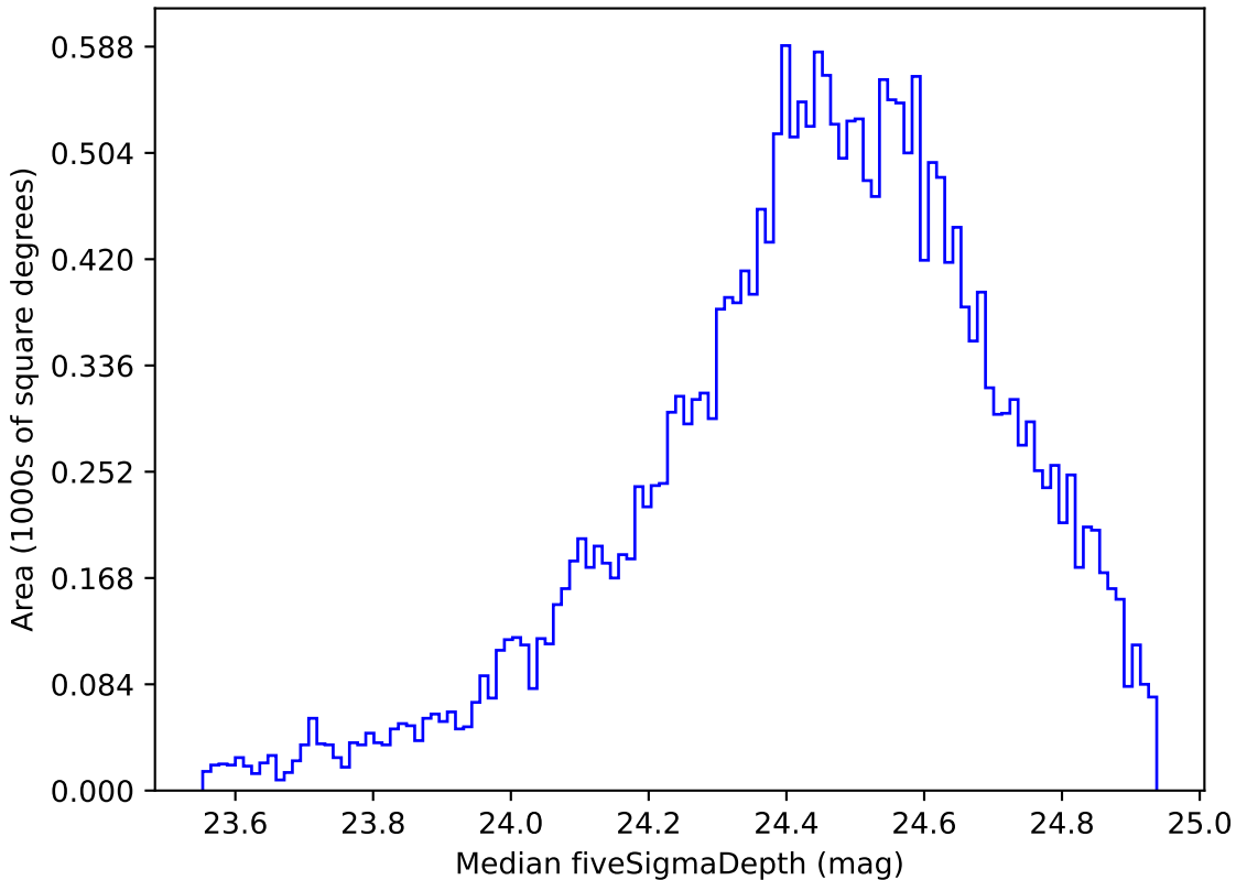
baseline_v3.0_10yrs Yr 1 g band: Median fiveSigmaDepth
