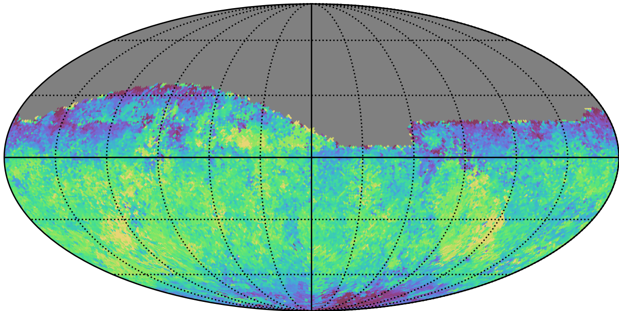
baseline_v3.0_10yrs Yr 1 all bands: Median fiveSigmaDepth
