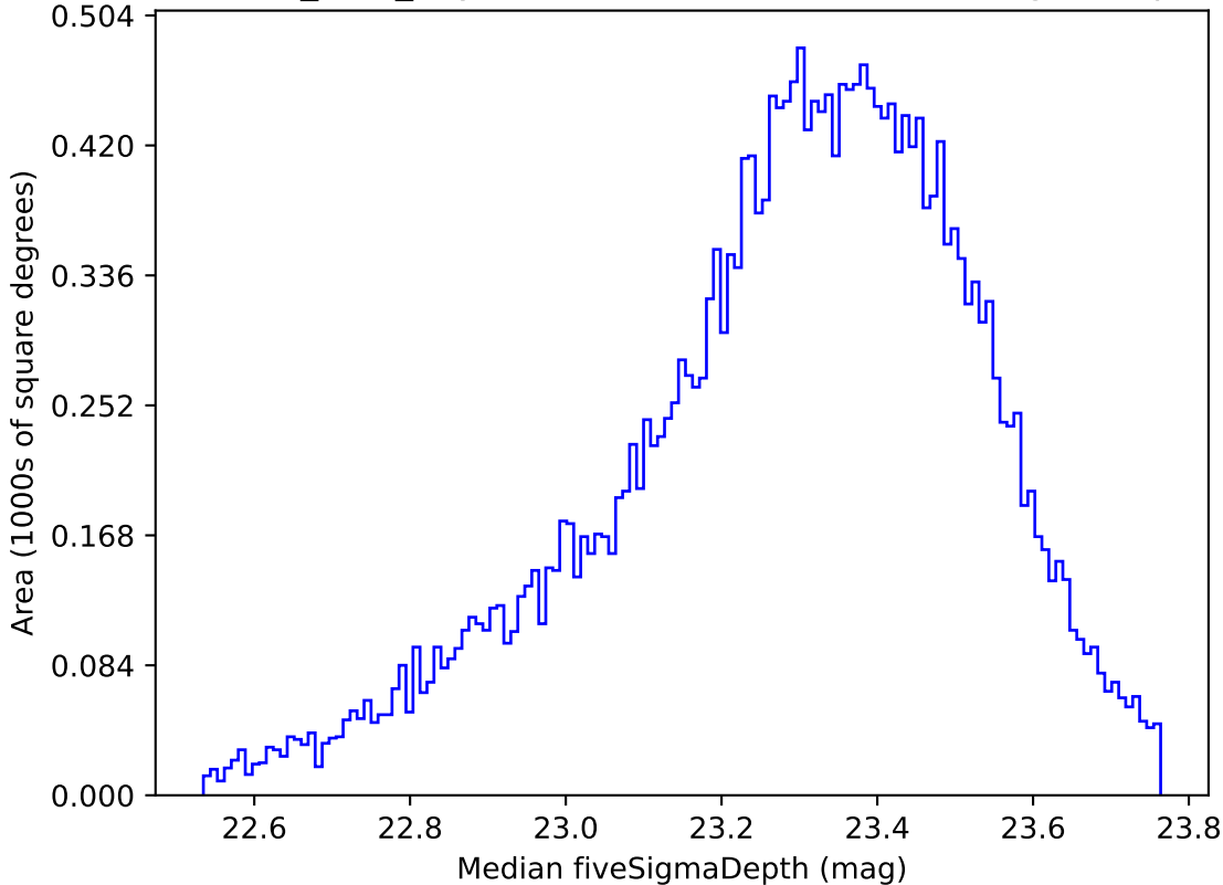
baseline_v3.0_10yrs Yr 1 all bands: Median fiveSigmaDepth
