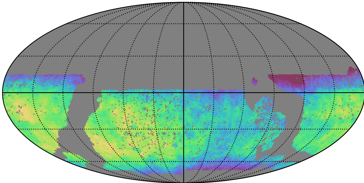
baseline_v3.0_10yrs WFD z band: Median fiveSigmaDepth
