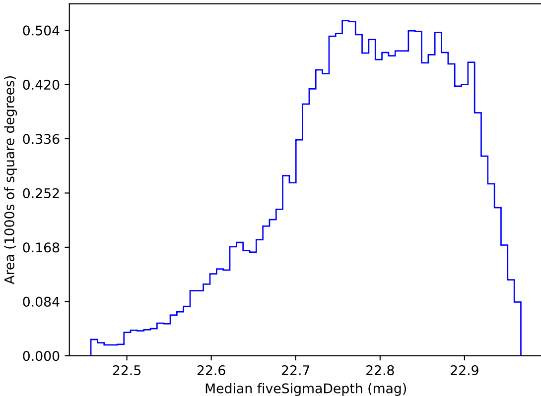
baseline_v3.0_10yrs WFD z band: Median fiveSigmaDepth
