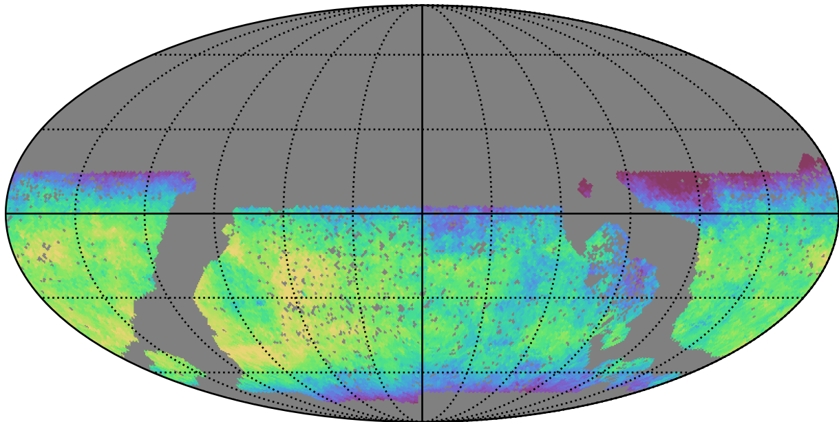
baseline_v3.0_10yrs WFD y band: Median fiveSigmaDepth
