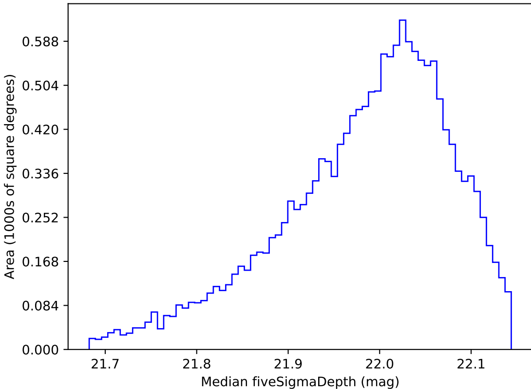
baseline_v3.0_10yrs WFD y band: Median fiveSigmaDepth
