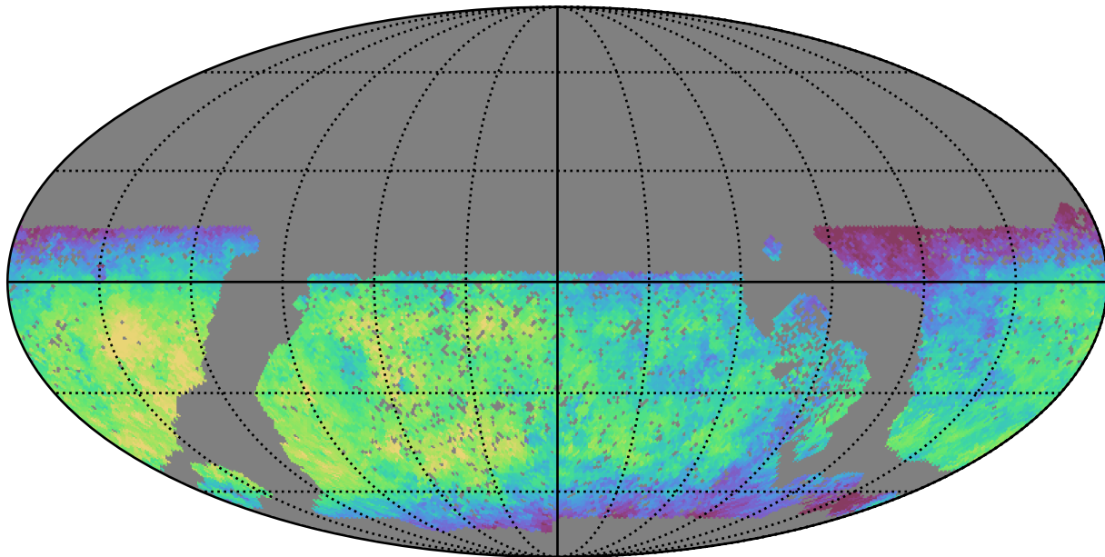
baseline_v3.0_10yrs WFD u band: Median fiveSigmaDepth
