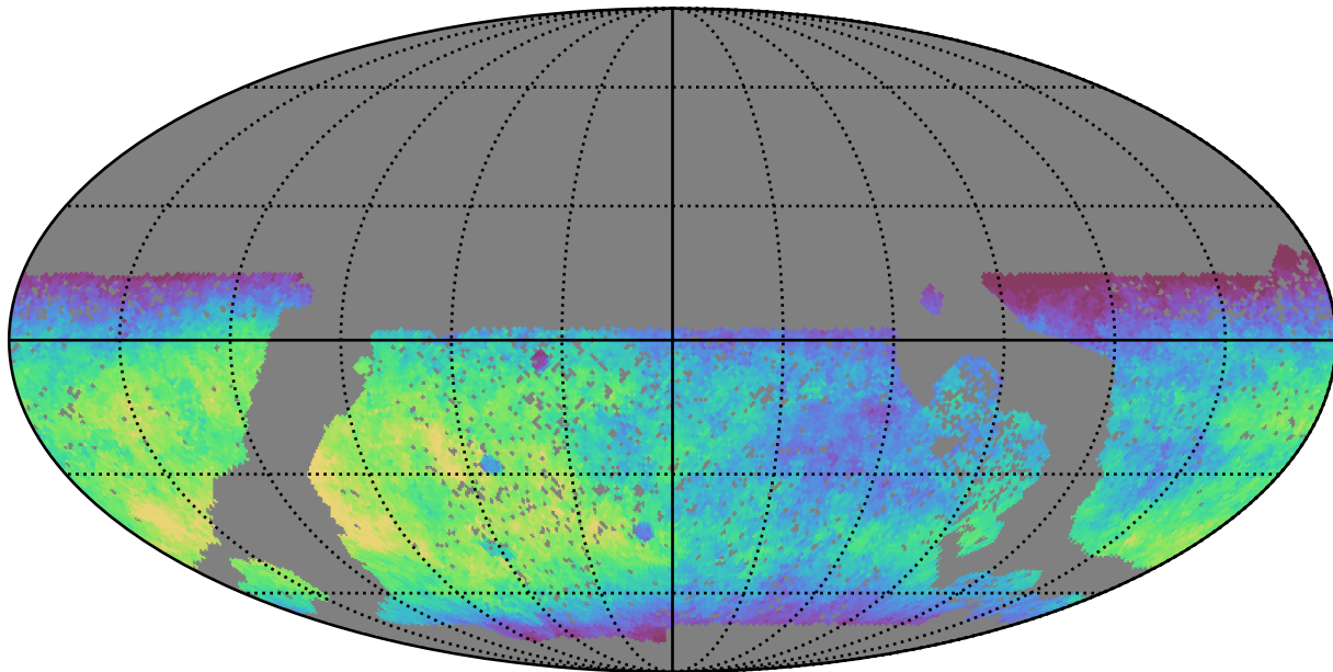
baseline_v3.0_10yrs WFD r band: Median fiveSigmaDepth
