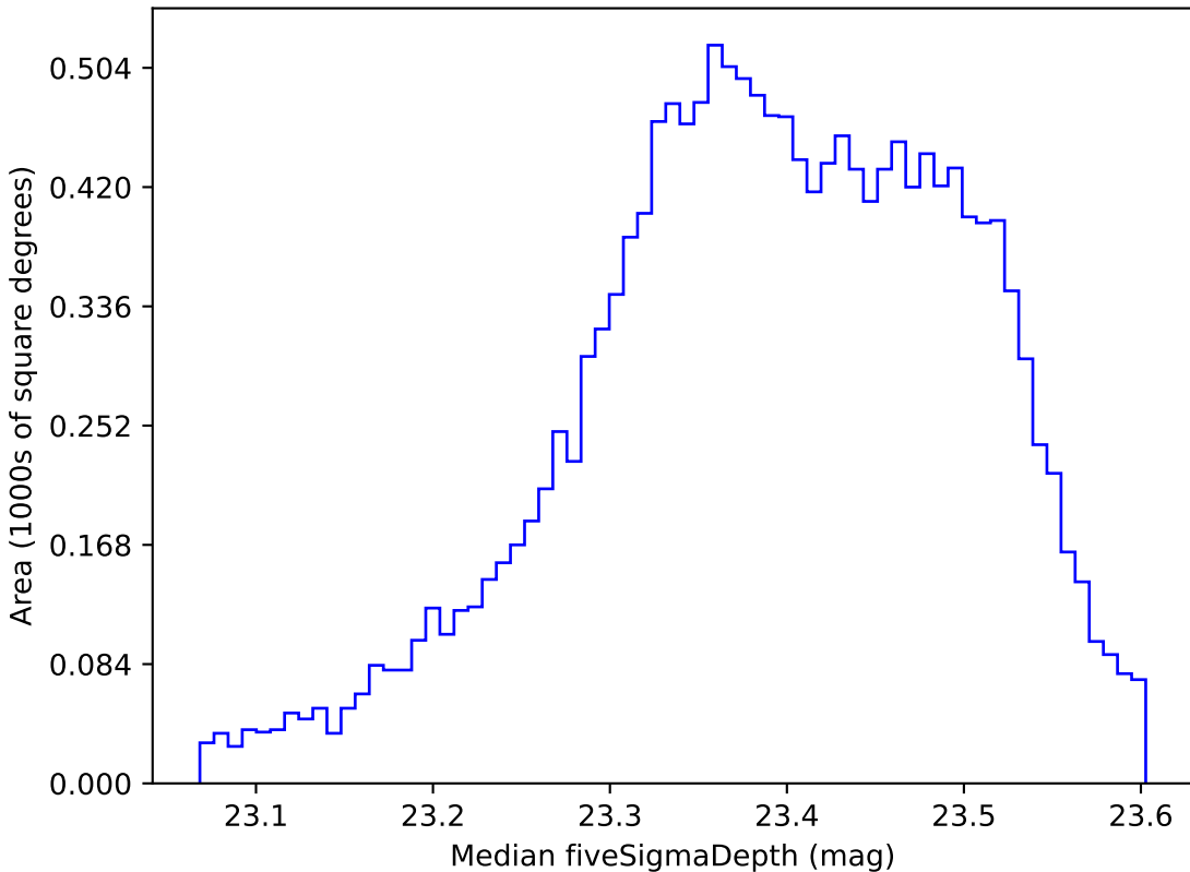
baseline_v3.0_10yrs WFD i band: Median fiveSigmaDepth
