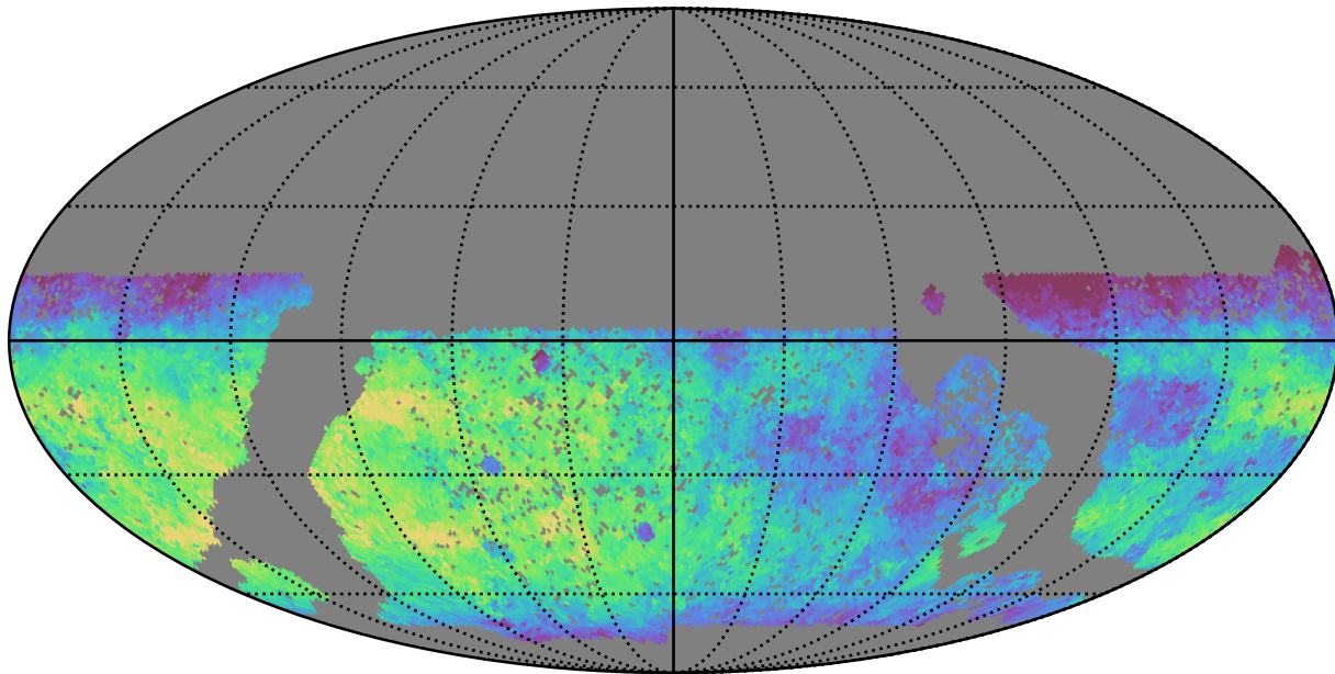
baseline_v3.0_10yrs WFD g band: Median fiveSigmaDepth
