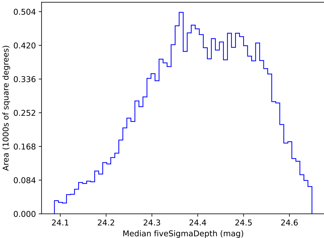
baseline_v3.0_10yrs WFD g band: Median fiveSigmaDepth
