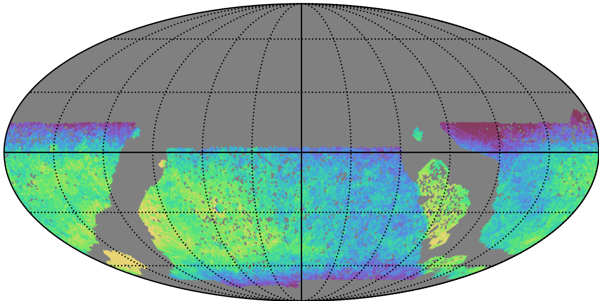
baseline_v3.0_10yrs WFD all bands: Median fiveSigmaDepth
