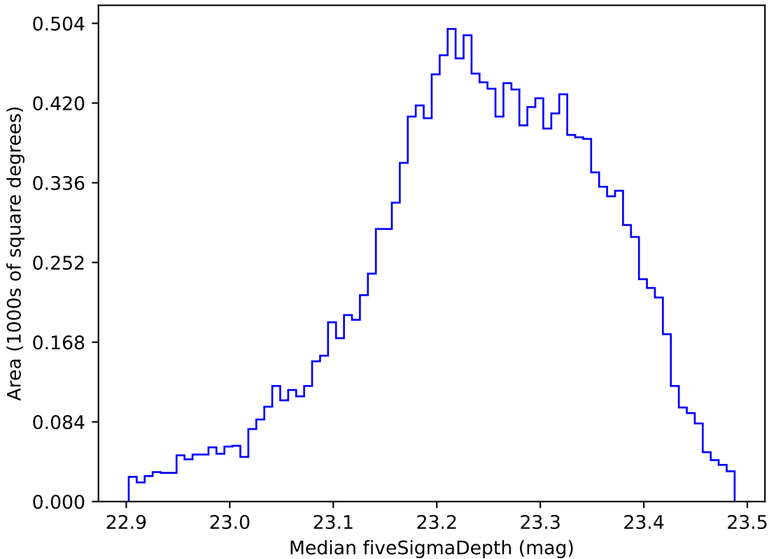
baseline_v3.0_10yrs WFD all bands: Median fiveSigmaDepth
