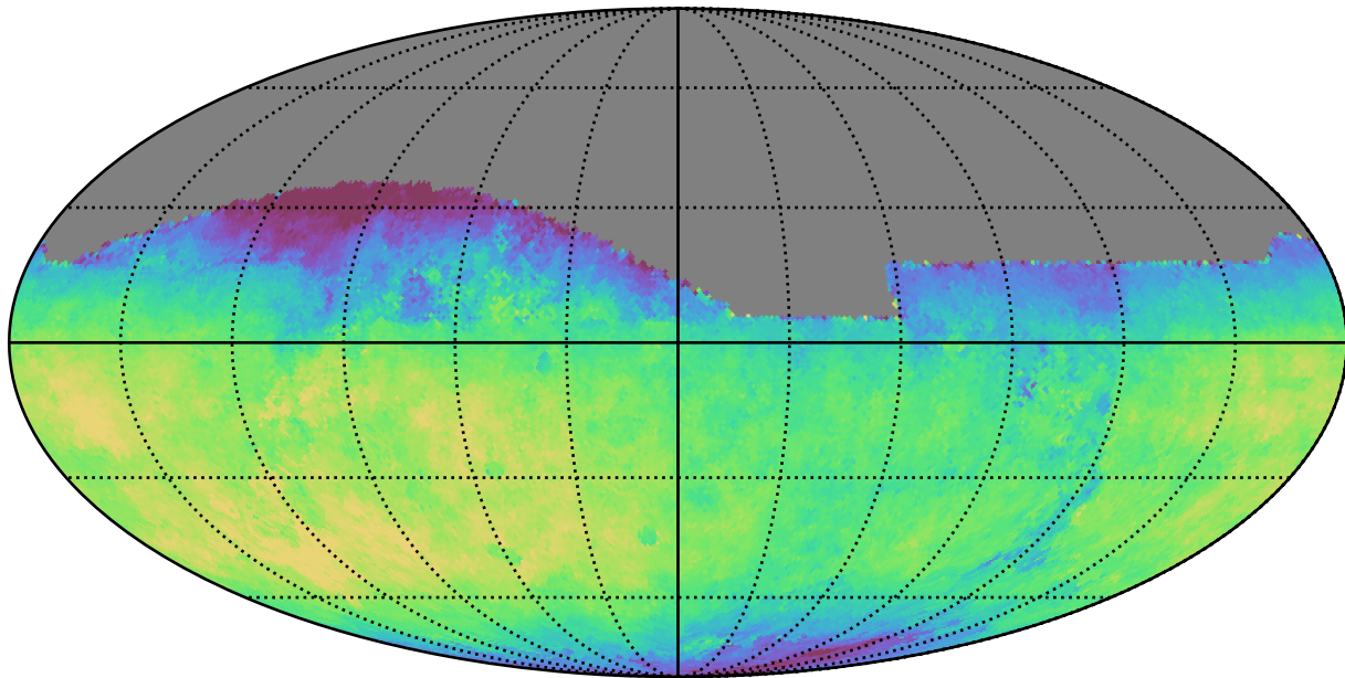
baseline_v3.0_10yrs All sky z band: Median fiveSigmaDepth
