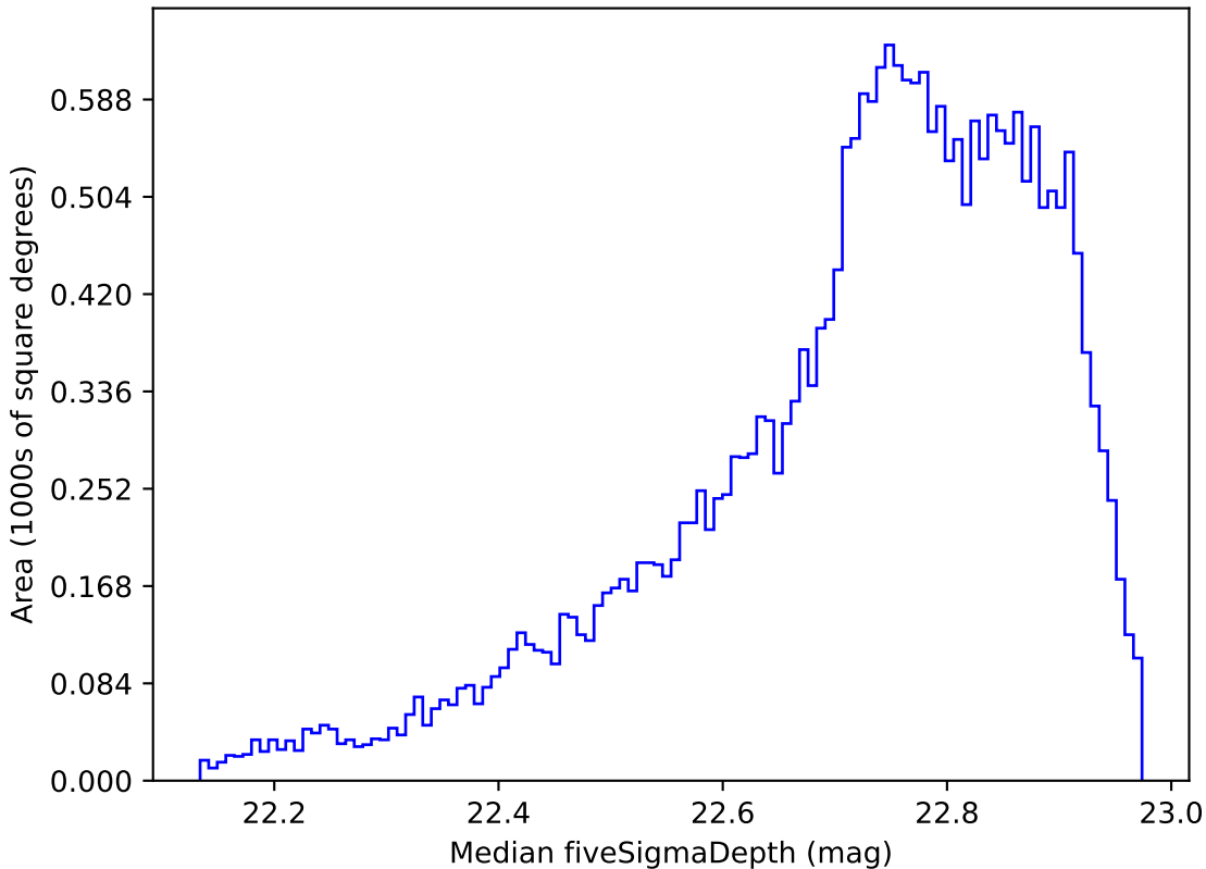
baseline_v3.0_10yrs All sky z band: Median fiveSigmaDepth
