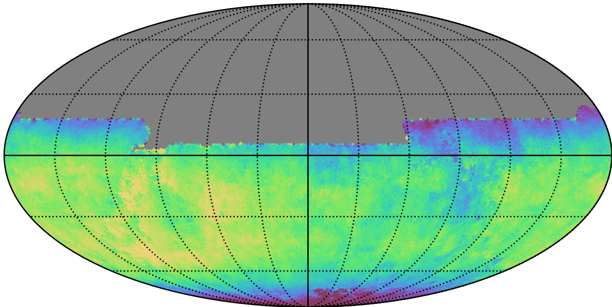
baseline_v3.0_10yrs All sky y band: Median fiveSigmaDepth
