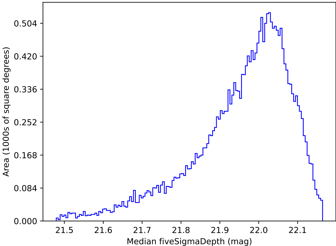
baseline_v3.0_10yrs All sky y band: Median fiveSigmaDepth
