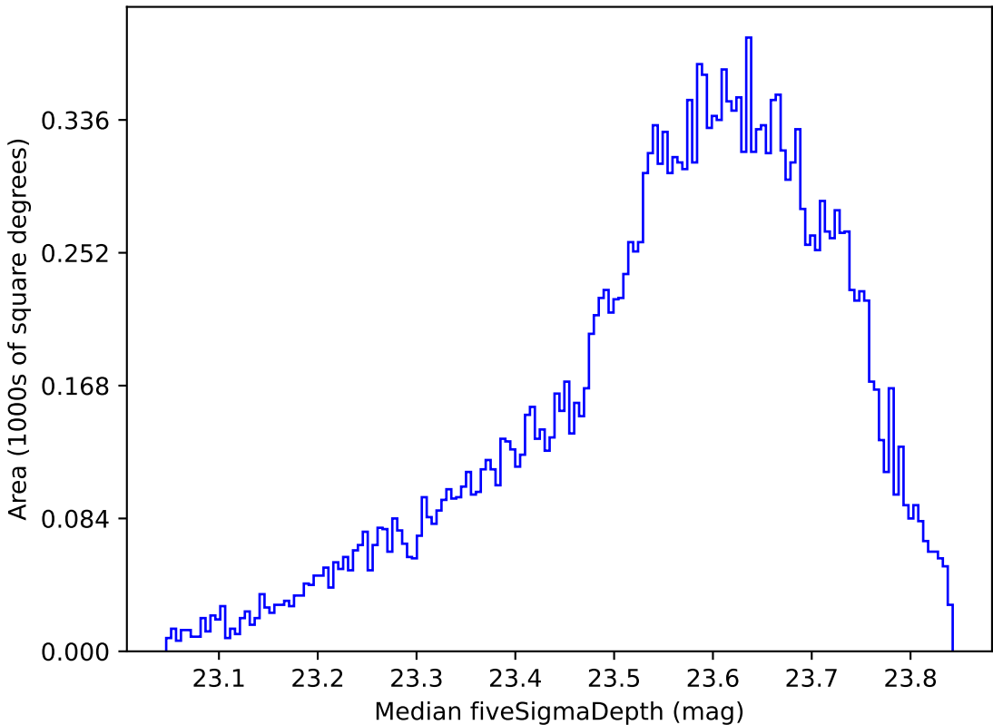
baseline_v3.0_10yrs All sky u band: Median fiveSigmaDepth
