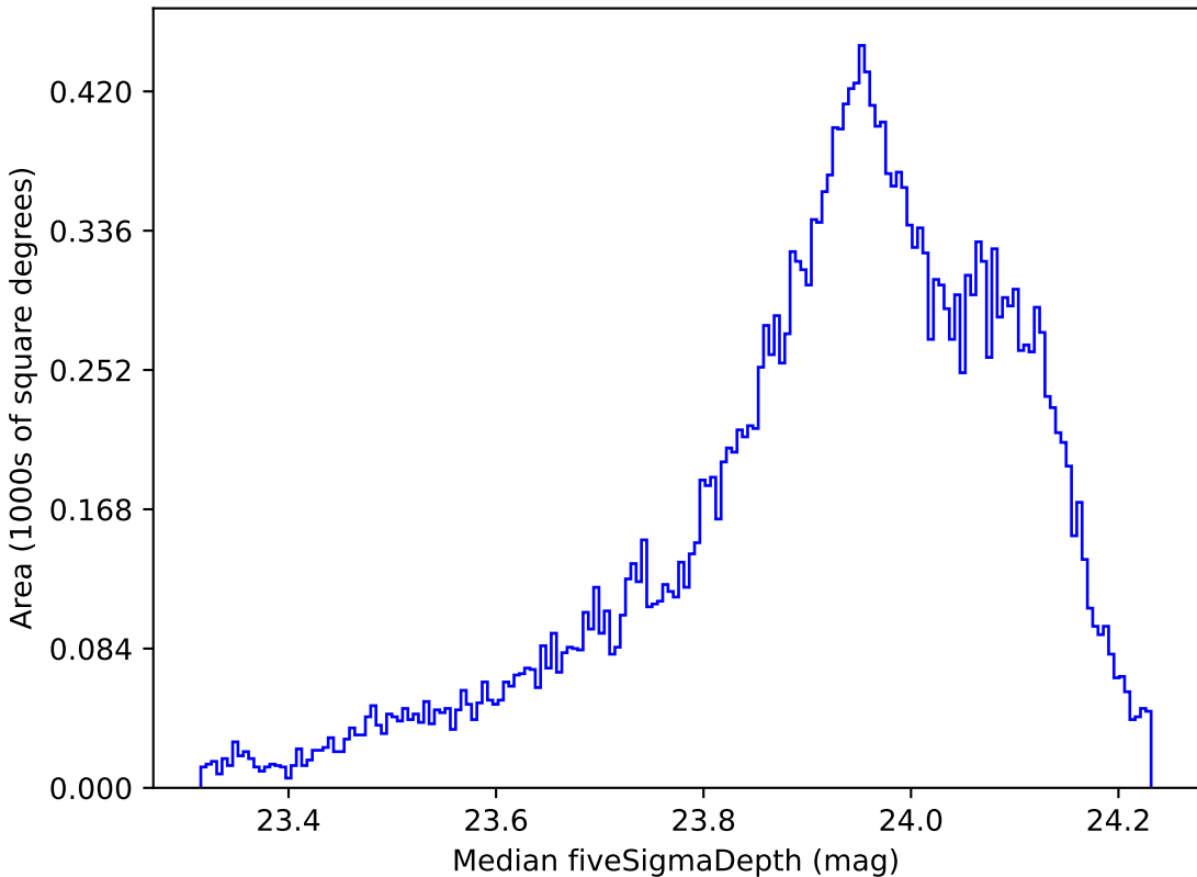
baseline_v3.0_10yrs All sky r band: Median fiveSigmaDepth
